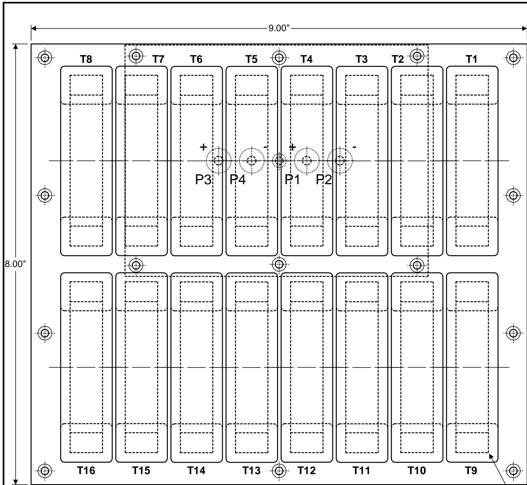
TOP VIEW (SECONDARY COIL CIRCUIT BOARD NOT SHOWN)
